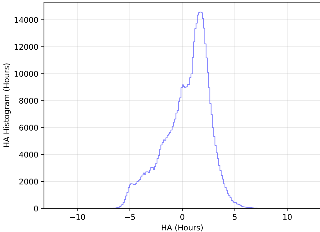
ddf_loaded_half_fl4_v3.4_10yrs WFD r band: HA Histogram
