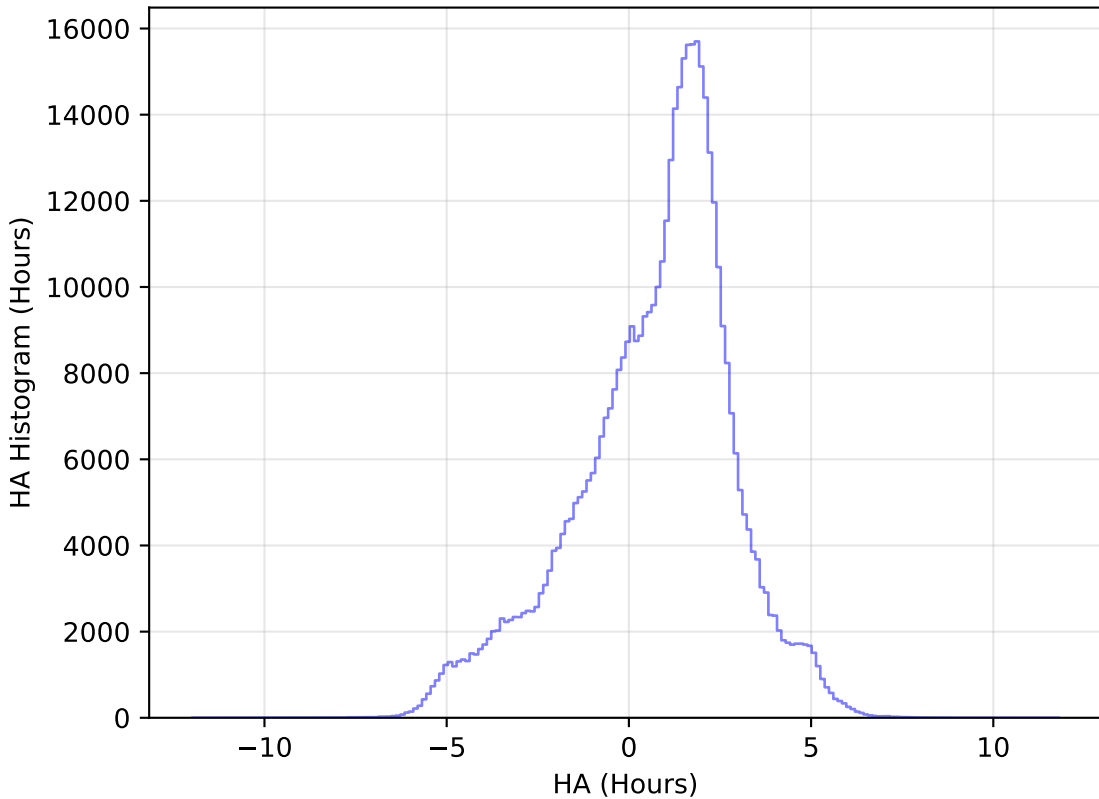
ddf_loaded_half_fl4_v3.4_10yrs WFD i band: HA Histogram
