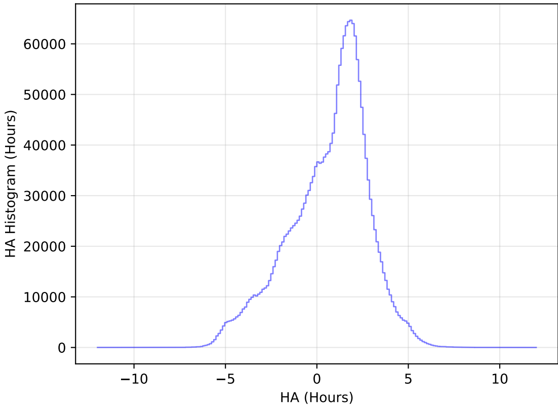
ddf_loaded_half_fl4_v3.4_10yrs WFD all bands: HA Histogram
