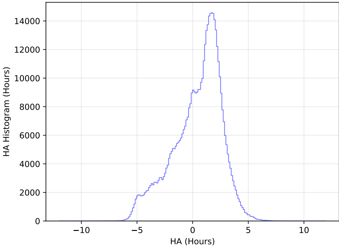
ddf_loaded_half_fl4_v3.4_10yrs All sky r band: HA Histogram
