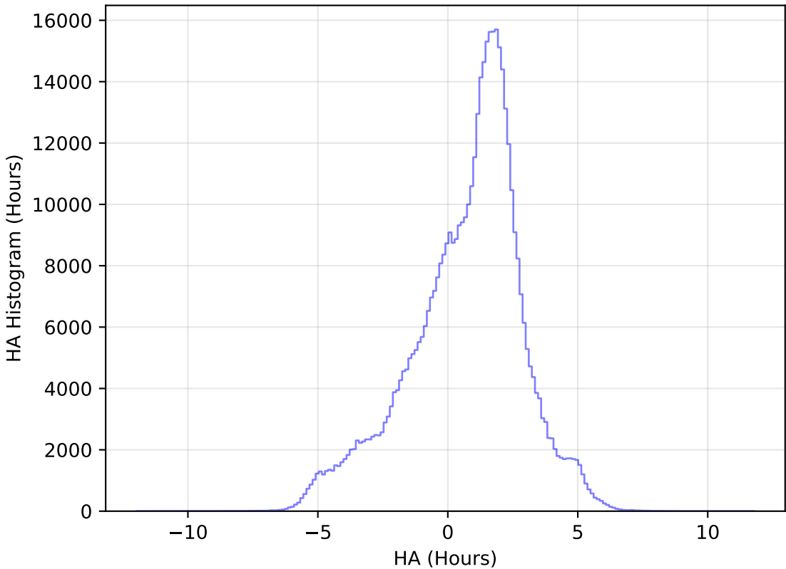
ddf_loaded_half_fl4_v3.4_10yrs All sky i band: HA Histogram
