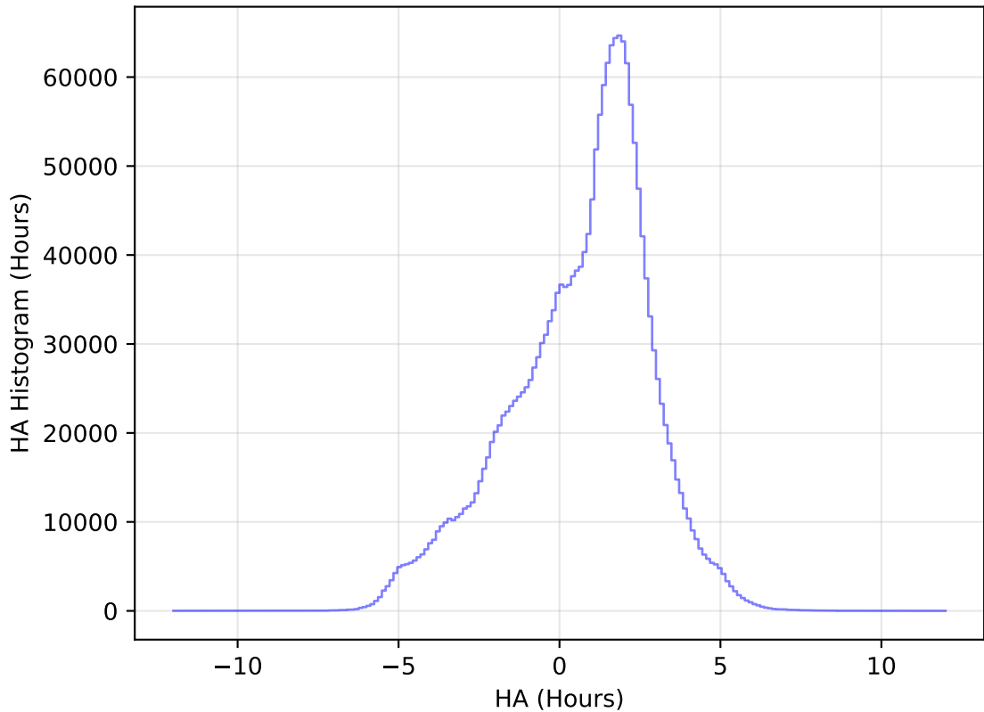
ddf_loaded_half_fl4_v3.4_10yrs All sky all bands: HA Histogram
