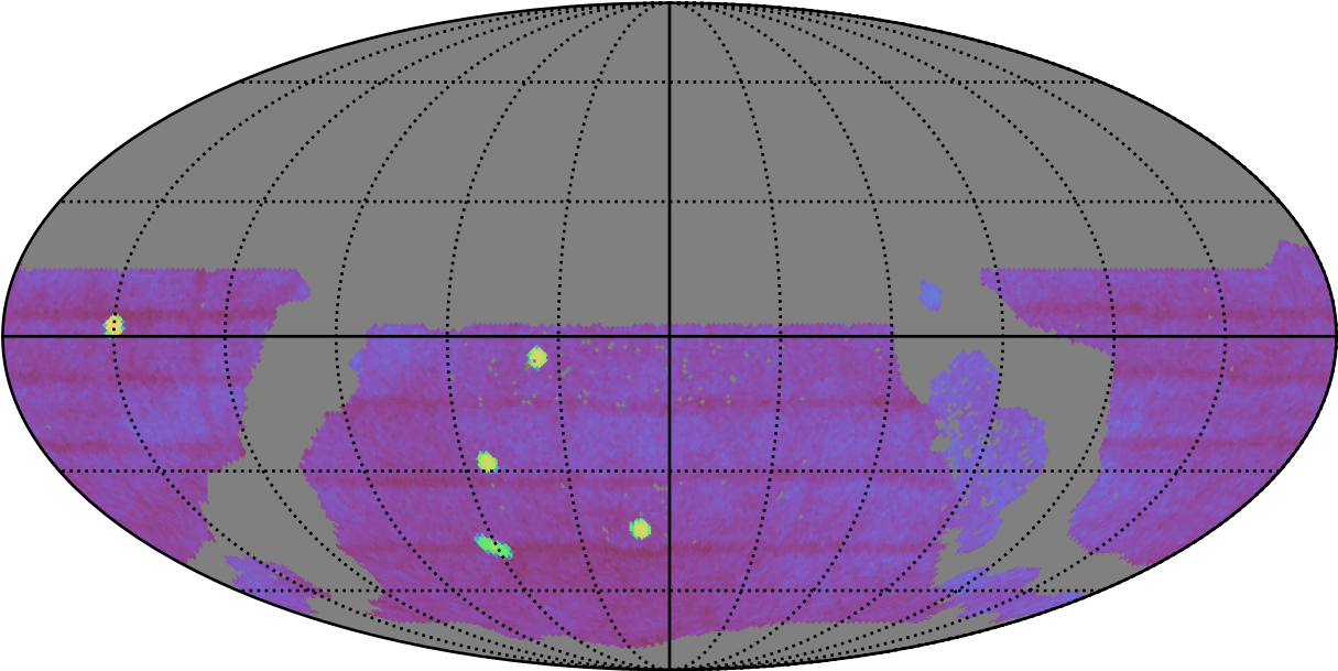
ddf_loaded_half_fl4_v3.4_10yrs gri WFD: Fraction of visits with a revisit < 60 min
