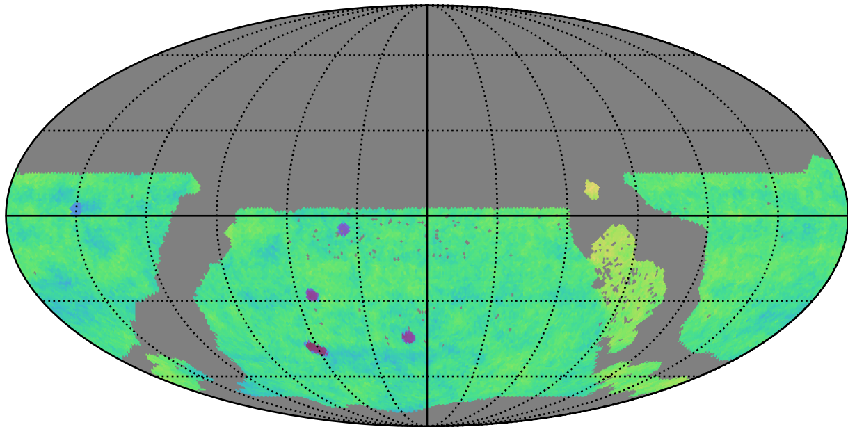
ddf_loaded_half_fl4_v3.4_10yrs gri WFD: Fraction of visits in pairs (10-60 min)
