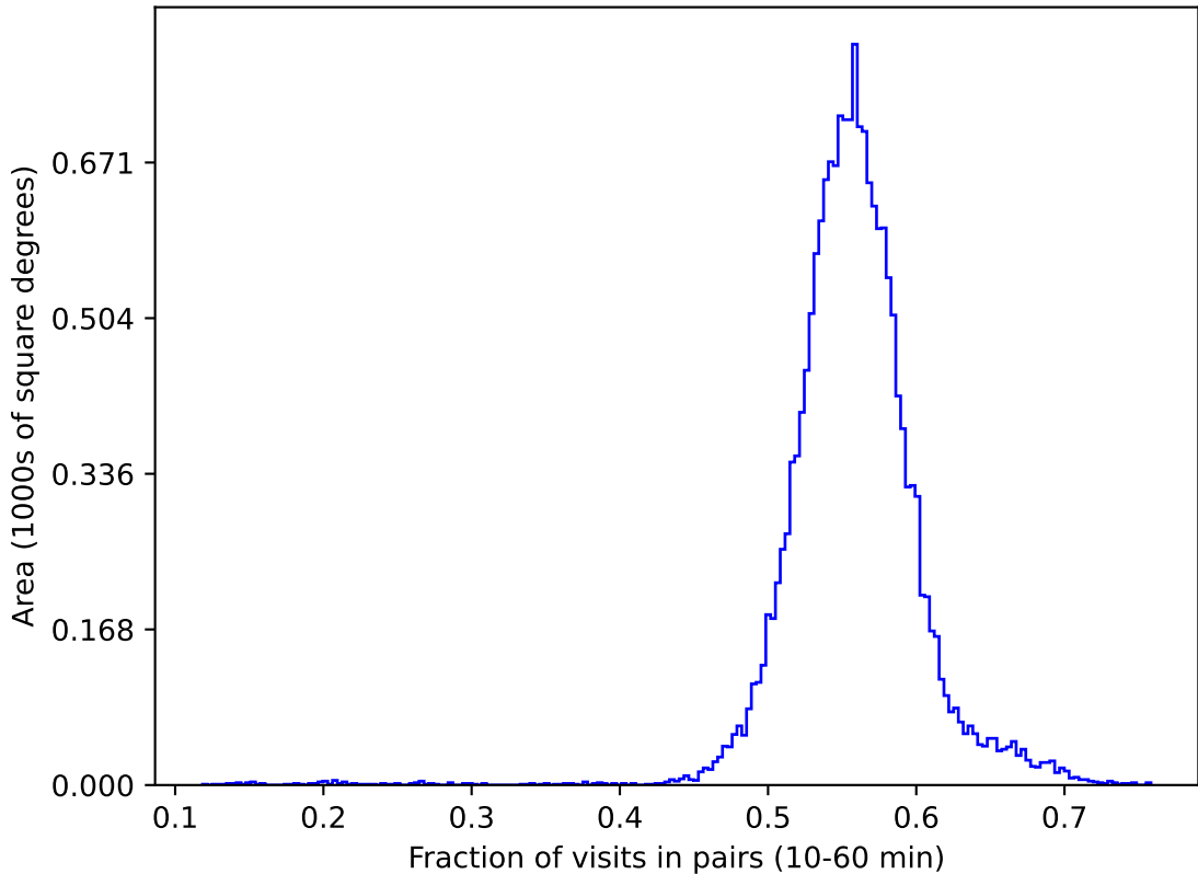
ddf_loaded_half_fl4_v3.4_10yrs gri WFD: Fraction of visits in pairs (10-60 min)
