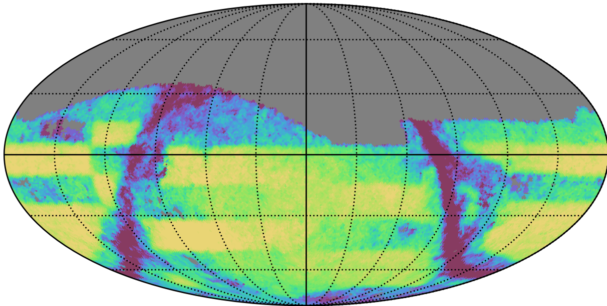
ddf_loaded_half_fl4_v3.4_10yrs Yr 3-4 i band: Exgal_CoaddM5
