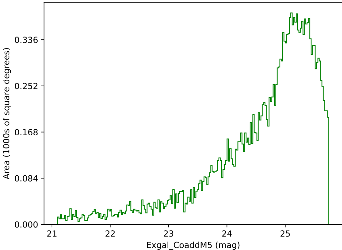
ddf_loaded_half_fl4_v3.4_10yrs Yr 3-4 g band: Exgal_CoaddM5
