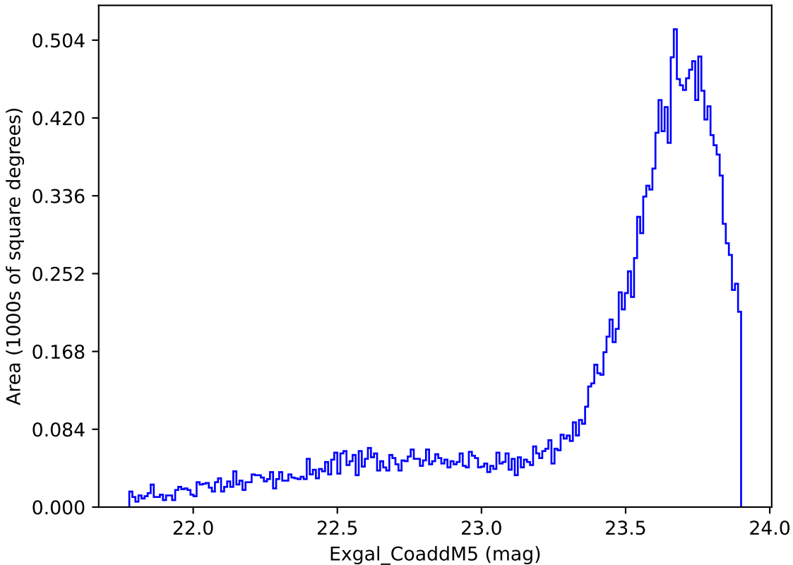
ddf_loaded_half_f14_v3.4_10yrs Yr 1 y band: Exgal_CoaddM5
