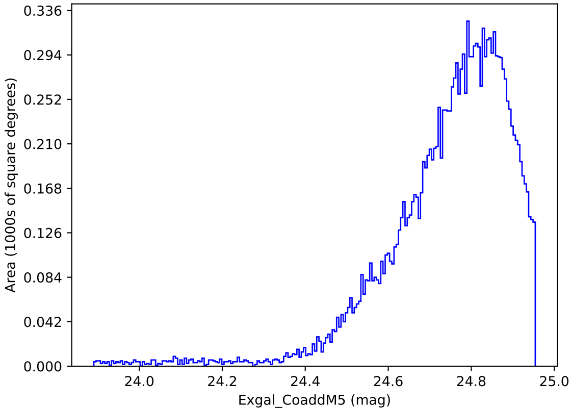
ddf_loaded_half_fl4_v3.4_10yrs WFD y band: Exgal_CoaddM5
