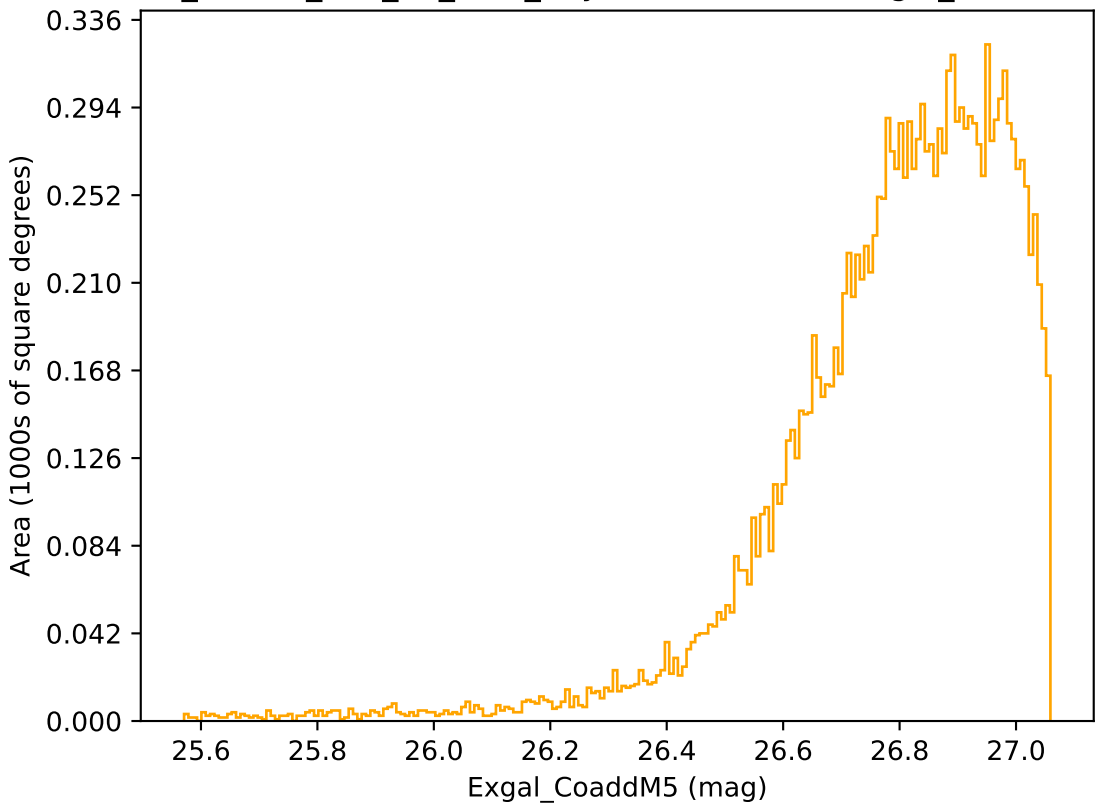
ddf_loaded_half_fl4_v3.4_10yrs WFD r band: Exgal_CoaddM5
