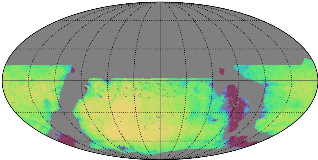
ddf_loaded_half_fl4_v3.4_10yrs WFD g band: Exgal_CoaddM5
