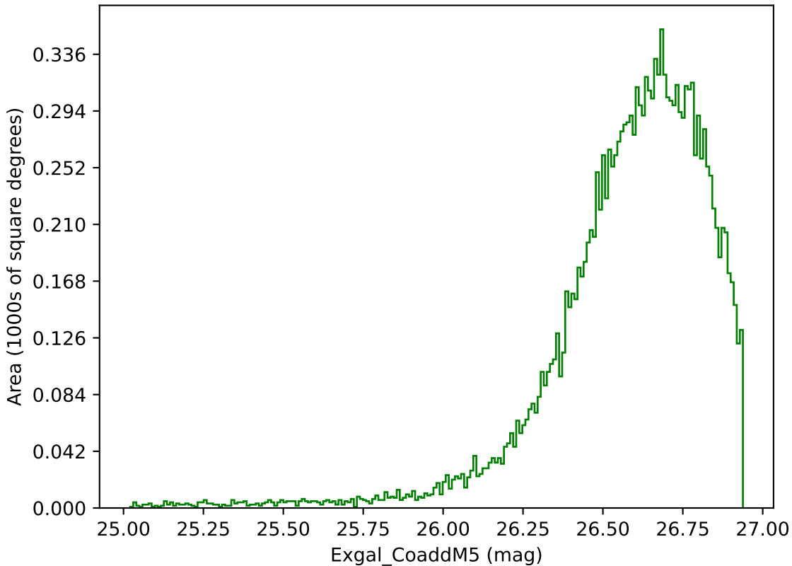
ddf_loaded_half_fl4_v3.4_10yrs WFD g band: Exgal_CoaddM5
