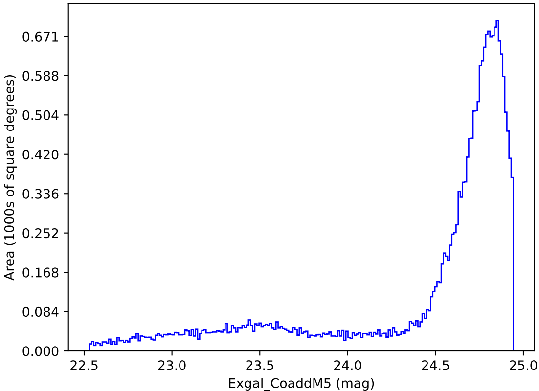
ddf_loaded_half_fl4_v3.4_10yrs All sky y band: Exgal_CoaddM5
