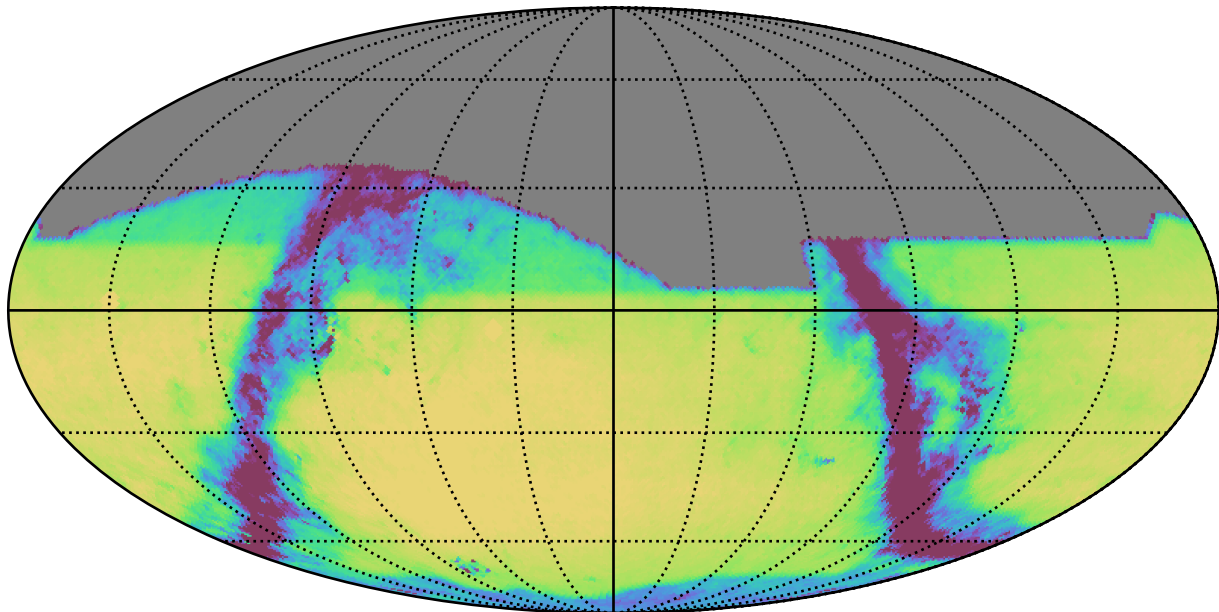
ddf_loaded_half_fl4_v3.4_10yrs All sky r band: Exgal_CoaddM5
