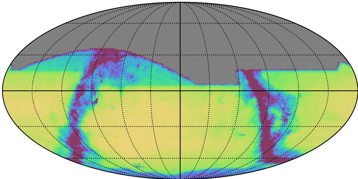
ddf_loaded_half_fl4_v3.4_10yrs All sky i band: Exgal_CoaddM5
