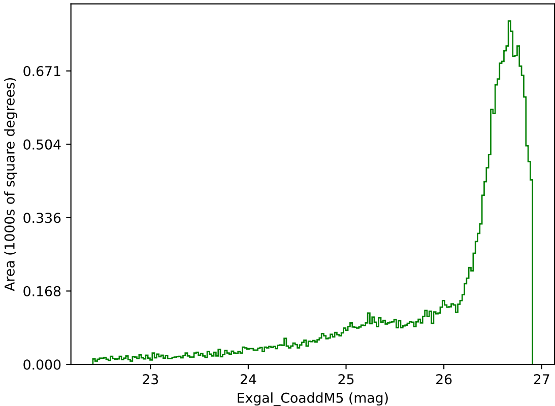
ddf_loaded_half_fl4_v3.4_10yrs All sky g band: Exgal_CoaddM5
