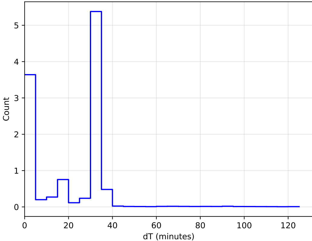
ddf_loaded_half_fl4_v3.4_10yrs WFD: DeltaT Histogram
