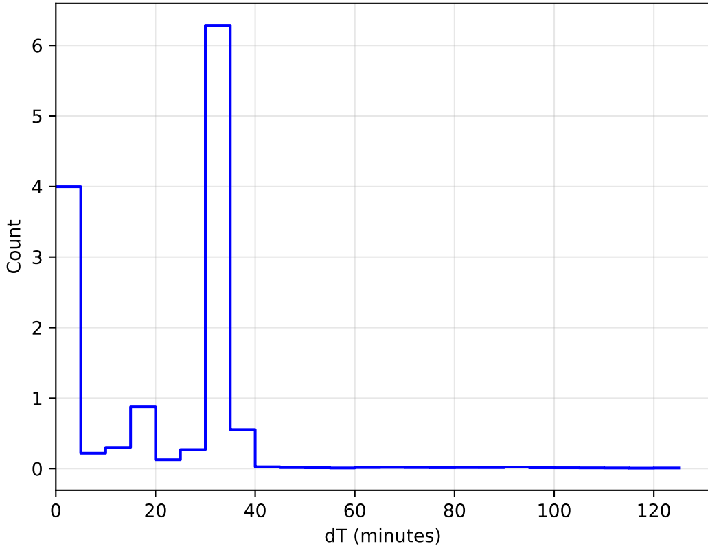
ddf_loaded_half_fl4_v3.4_10yrs All sky: DeltaT Histogram
