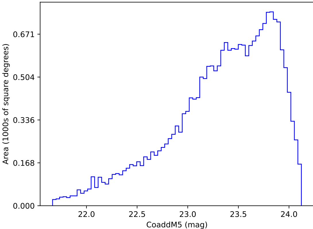
ddf_loaded_half_fl4_v3.4_10yrs Yr 3-4 y band: CoaddM5
