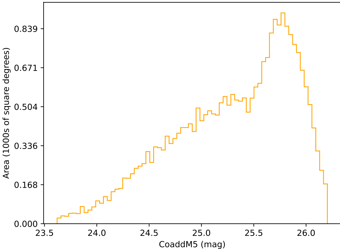
ddf_loaded_half_fl4_v3.4_10yrs Yr 3-4 r band: CoaddM5
