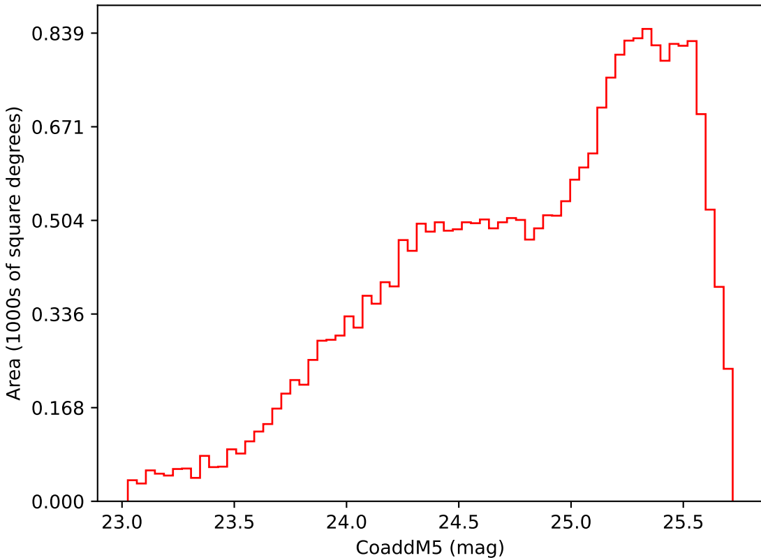
ddf_loaded_half_fl4_v3.4_10yrs Yr 3-4 i band: CoaddM5
