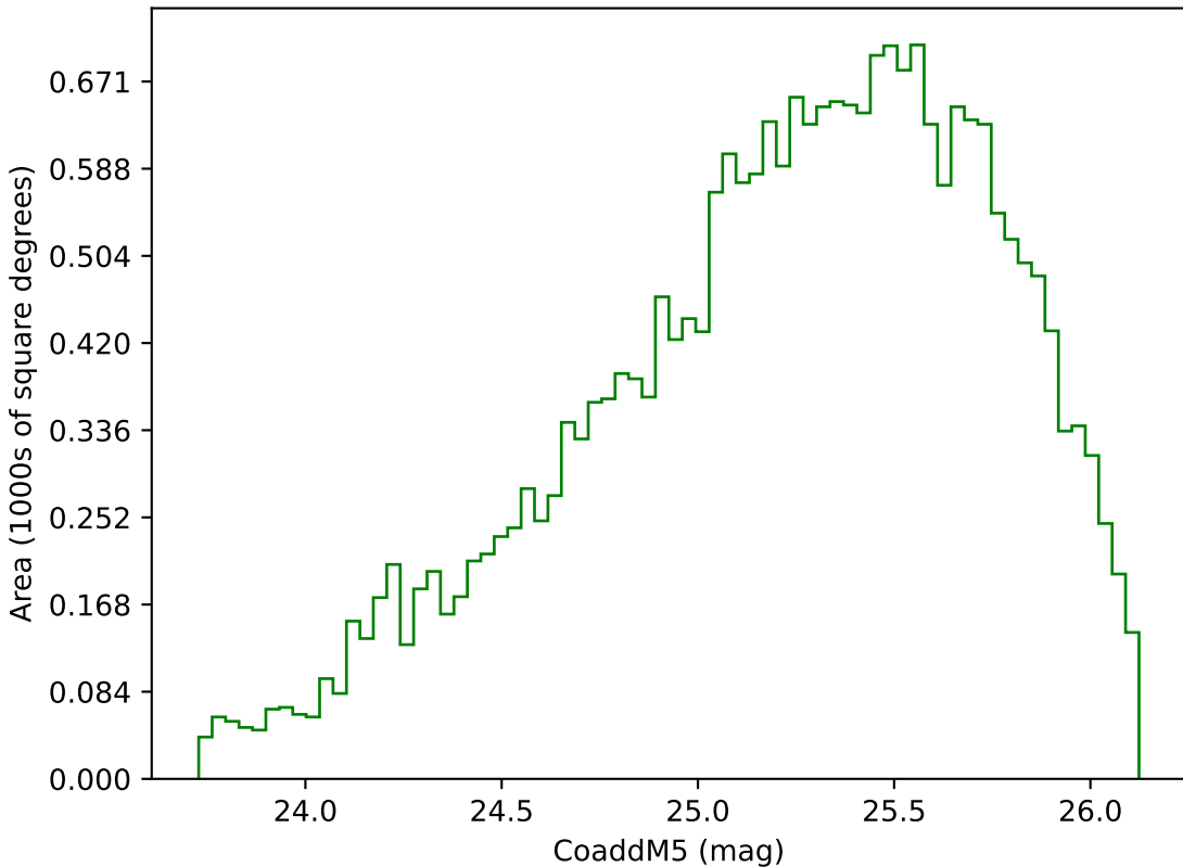
ddf_loaded_half_fl4_v3.4_10yrs Yr 3-4 g band: CoaddM5
