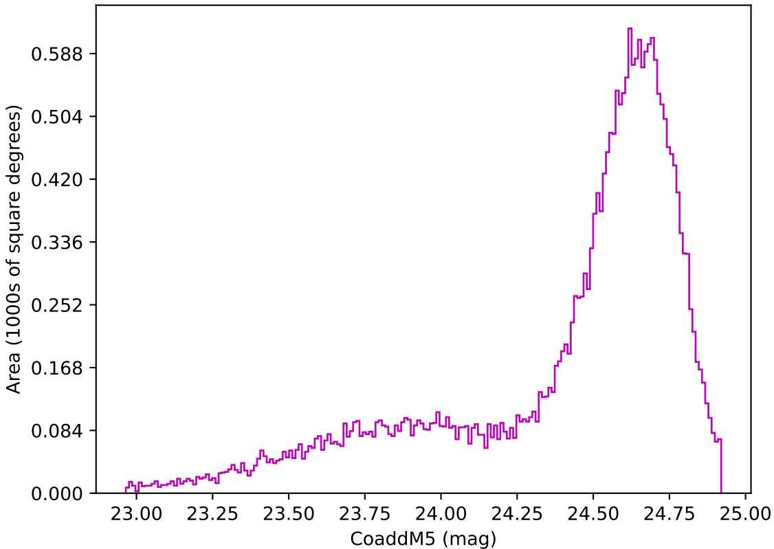
ddf_loaded_half_fl4_v3.4_10yrs Yr 1 z band: CoaddM5
