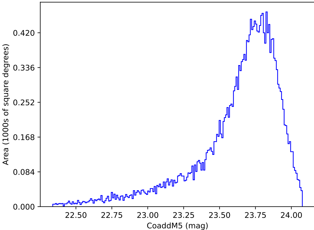
ddf_loaded_half_f14_v3.4_10yrs Yr 1 y band: CoaddM5
