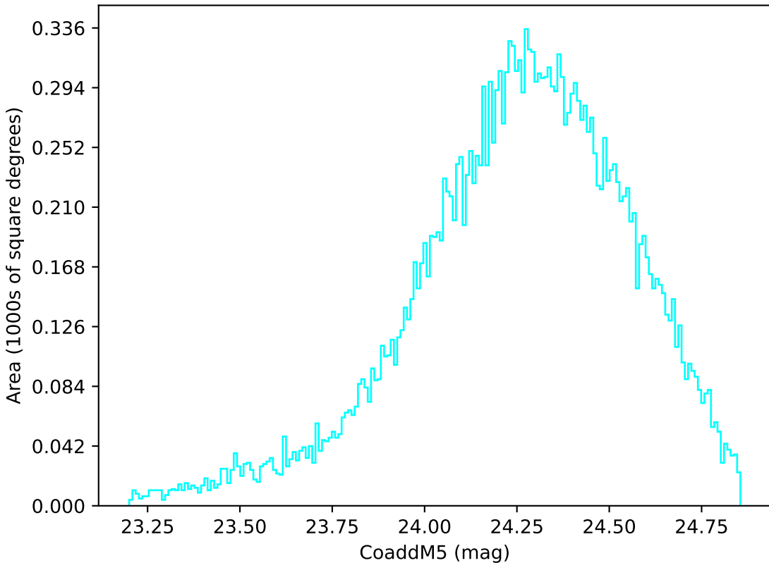
ddf_loaded_half_fl4_v3.4_10yrs Yr 1 u band: CoaddM5
