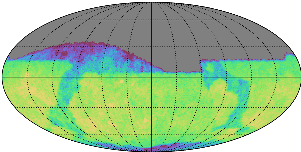
ddf_loaded_half_fl4_v3.4_10yrs Yr 1 r band: CoaddM5
