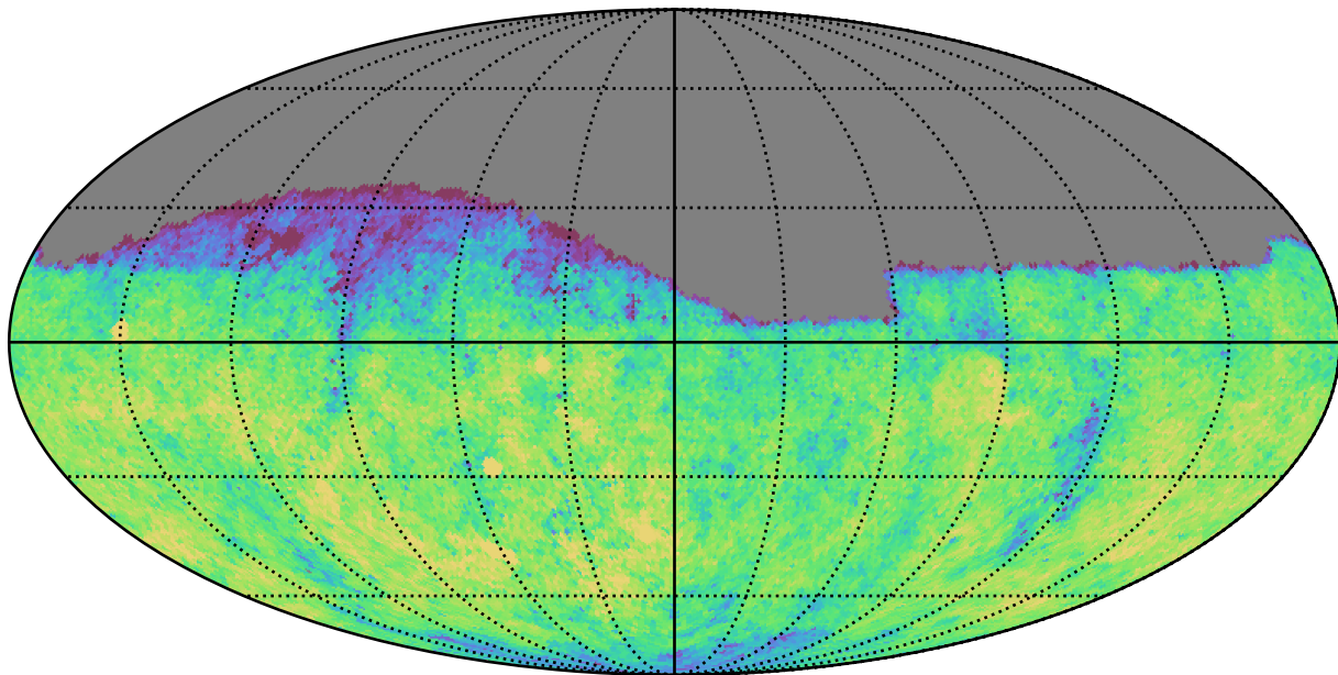
ddf_loaded_half_fl4_v3.4_10yrs Yr 1 g band: CoaddM5
