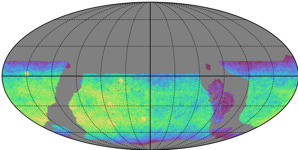
ddf_loaded_half_fl4_v3.4_10yrs WFD y band: CoaddM5
