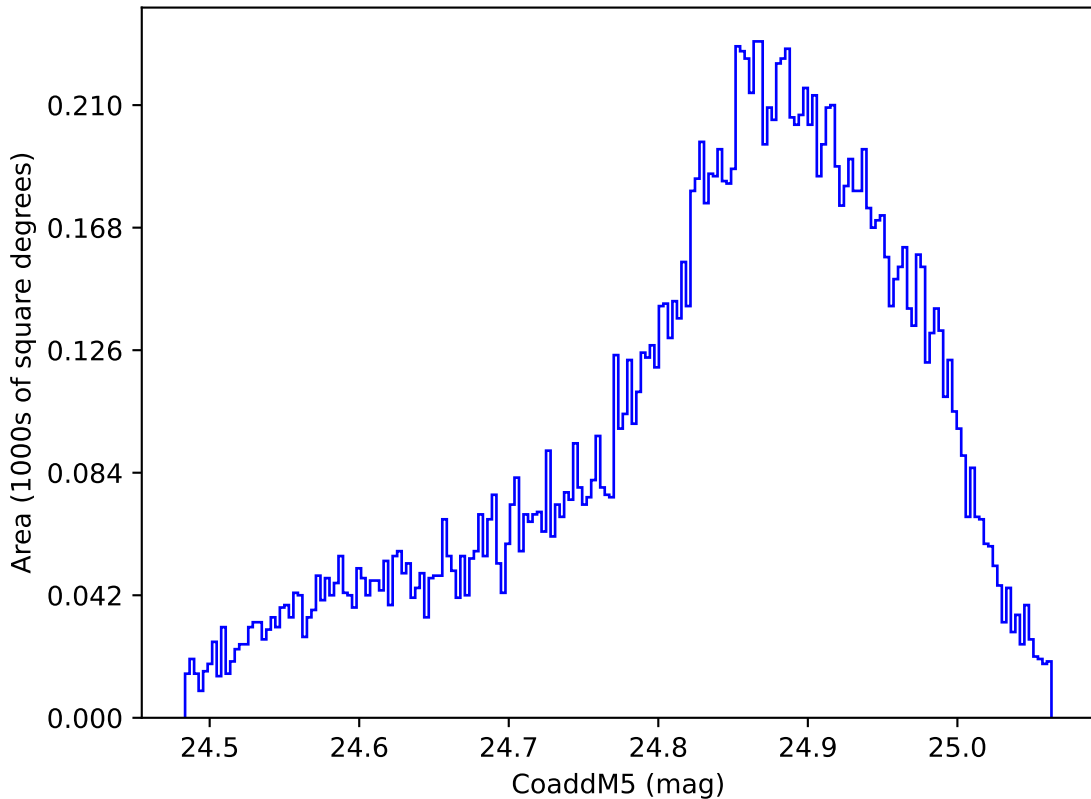
ddf_loaded_half_fl4_v3.4_10yrs WFD y band: CoaddM5
