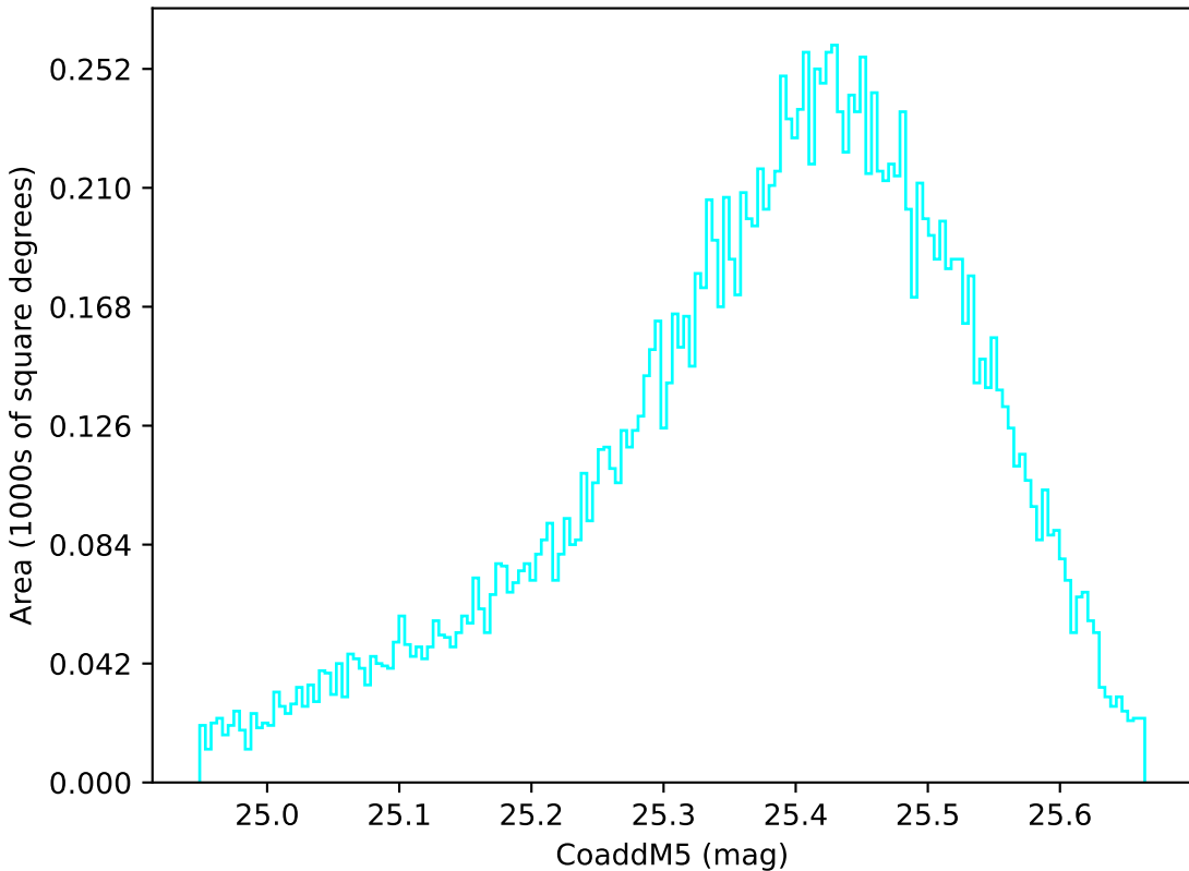
ddf_loaded_half_fl4_v3.4_10yrs WFD u band: CoaddM5
