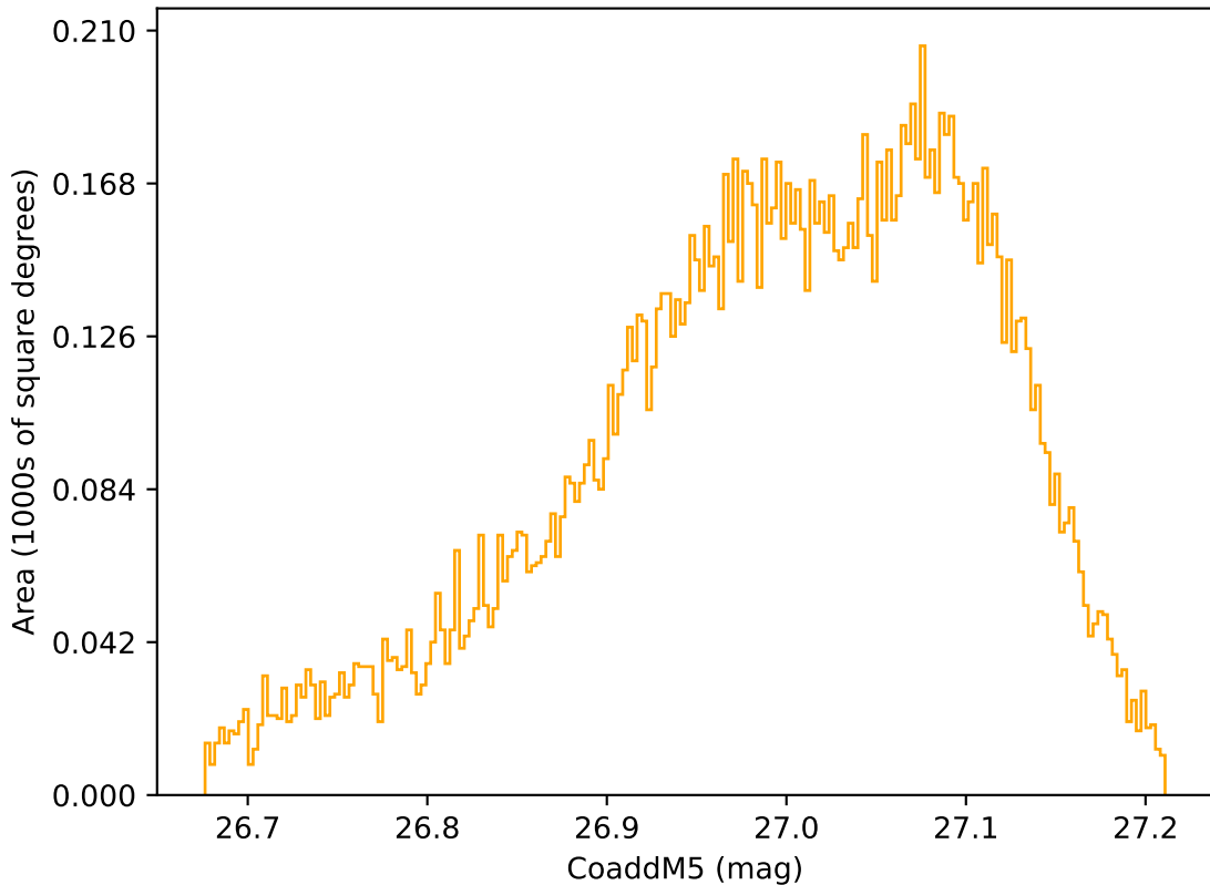
ddf_loaded_half_fl4_v3.4_10yrs WFD r band: CoaddM5
