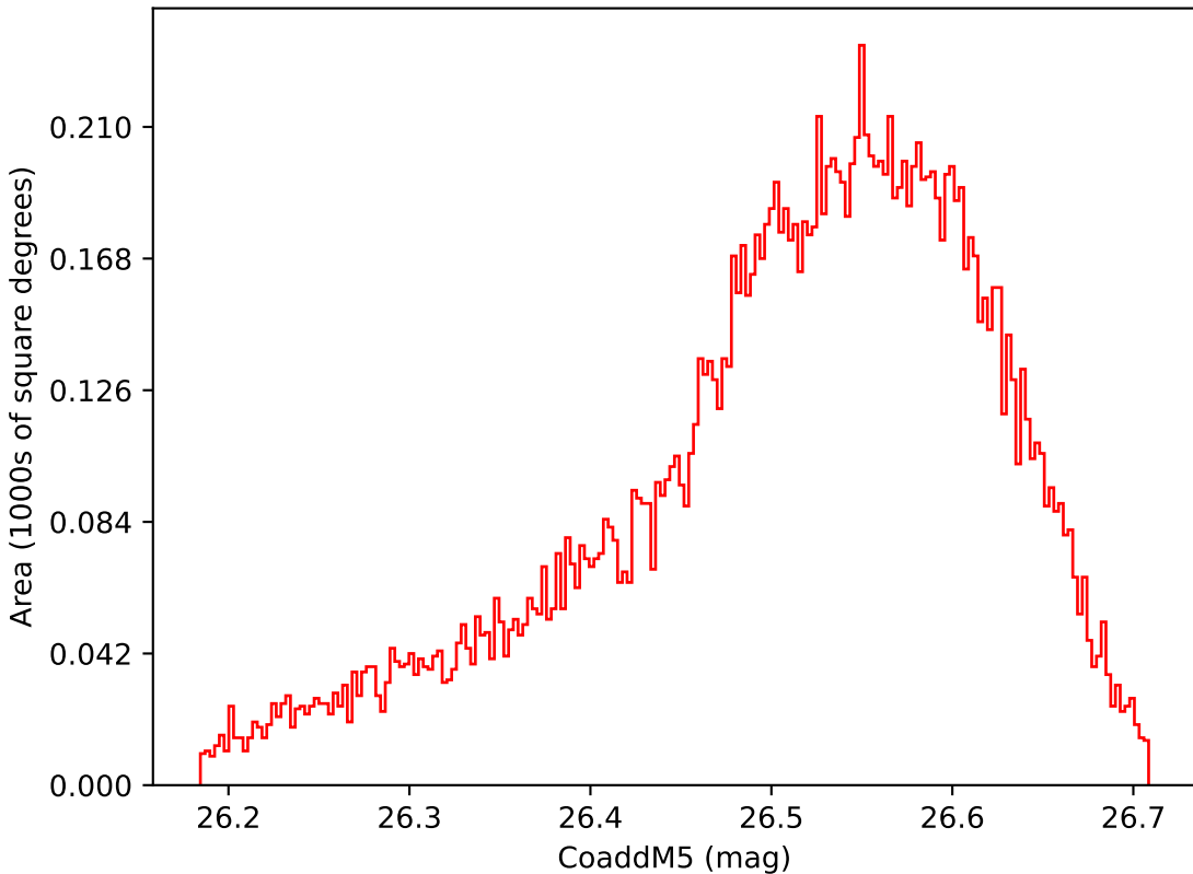
ddf_loaded_half_fl4_v3.4_10yrs WFD i band: CoaddM5
