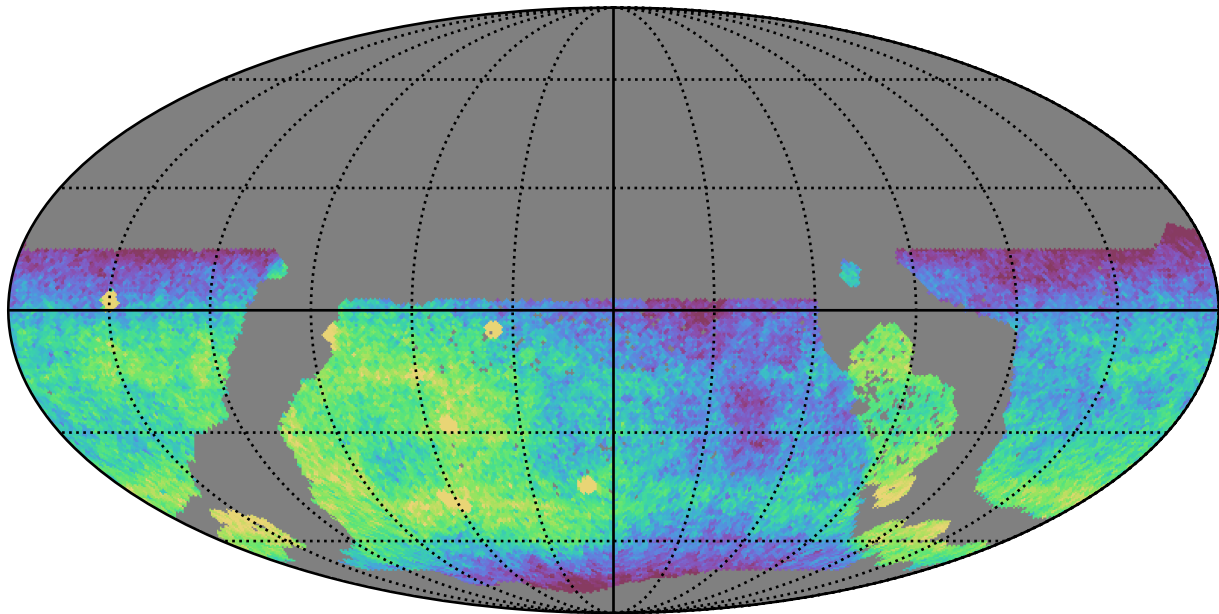
ddf_loaded_half_fl4_v3.4_10yrs WFD g band: CoaddM5
