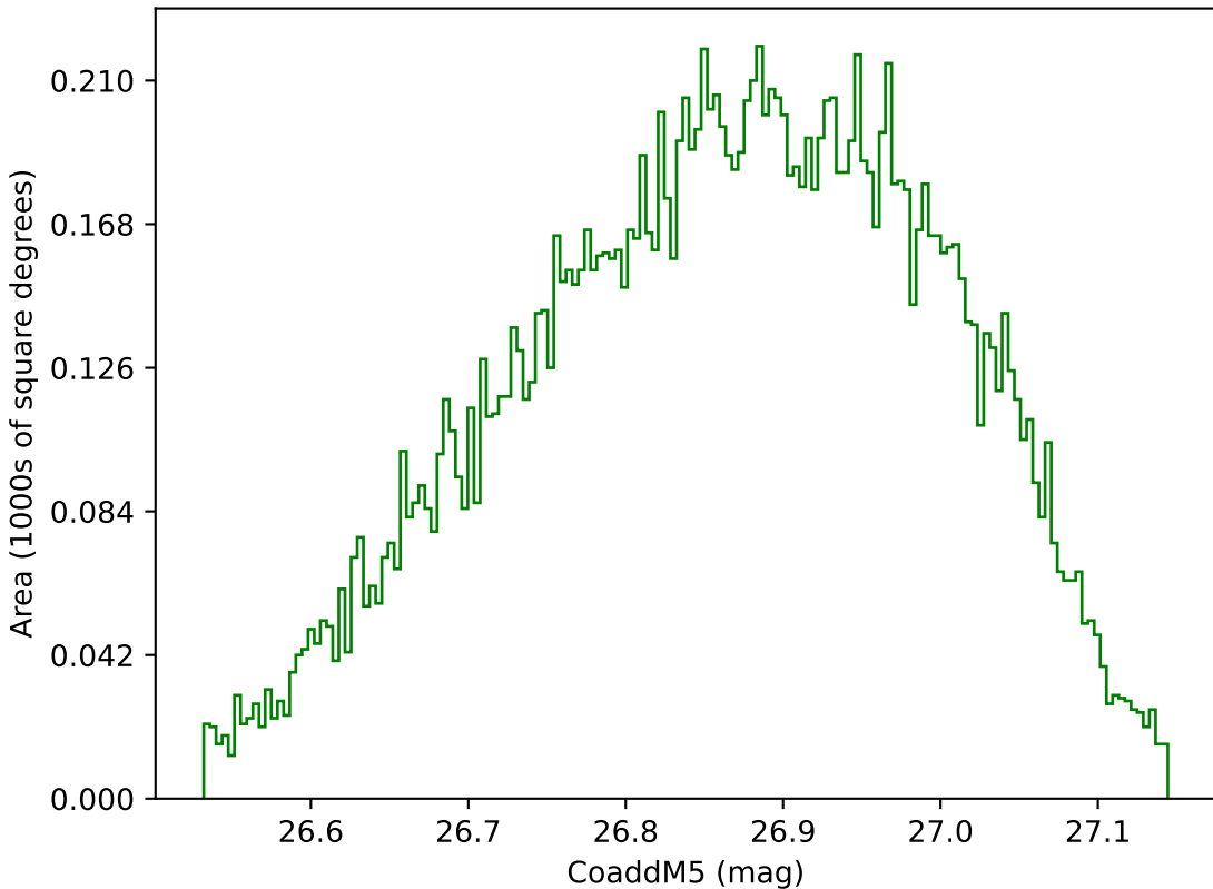
ddf_loaded_half_fl4_v3.4_10yrs WFD g band: CoaddM5
