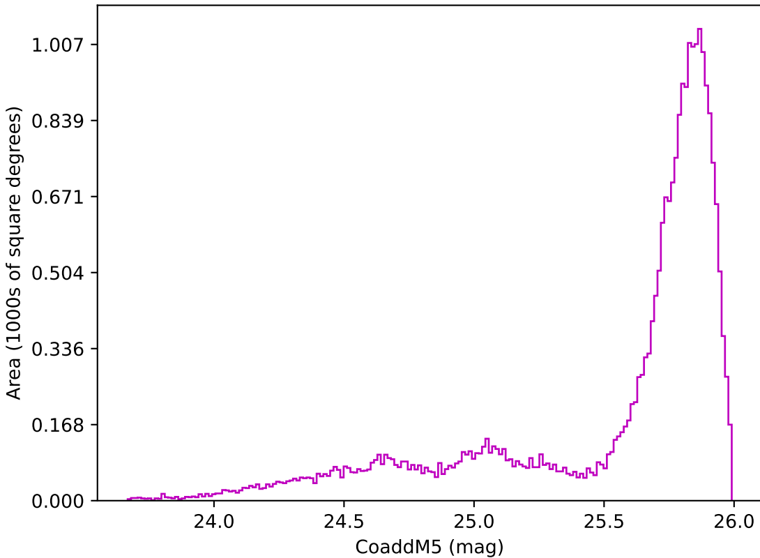
ddf_loaded_half_fl4_v3.4_10yrs All sky z band: CoaddM5
