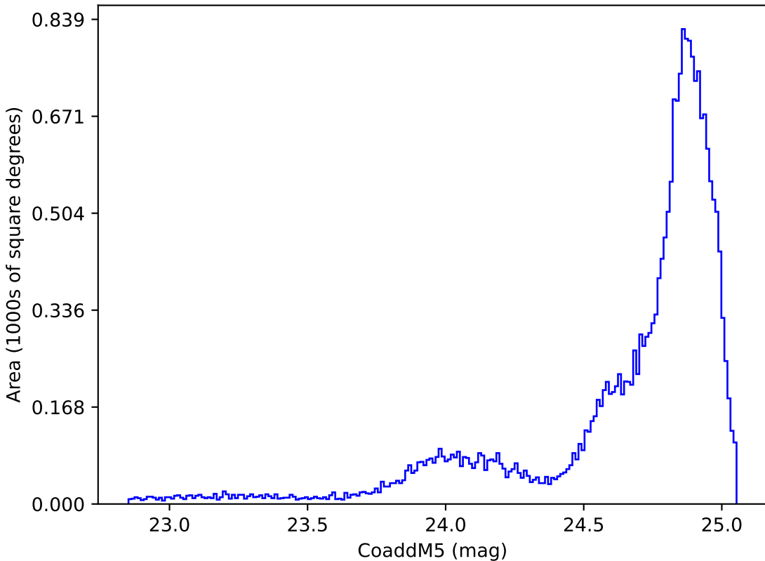
ddf_loaded_half_fl4_v3.4_10yrs All sky y band: CoaddM5
