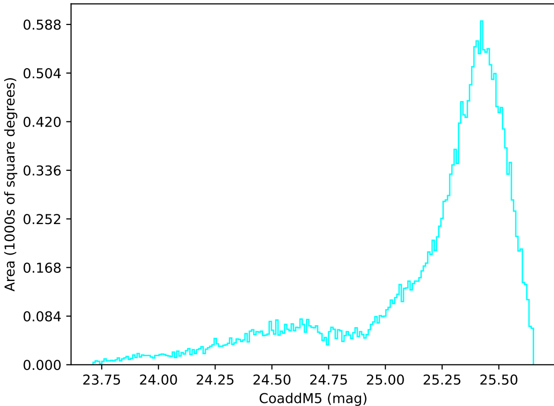
ddf_loaded_half_fl4_v3.4_10yrs All sky u band: CoaddM5
