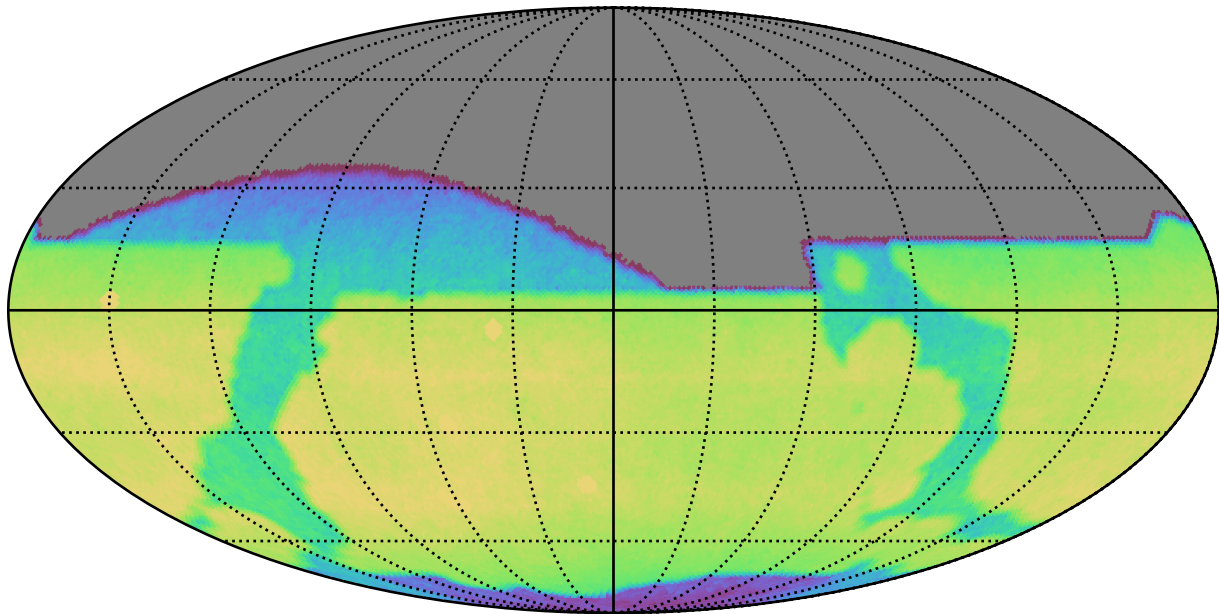
ddf_loaded_half_fl4_v3.4_10yrs All sky i band: CoaddM5
