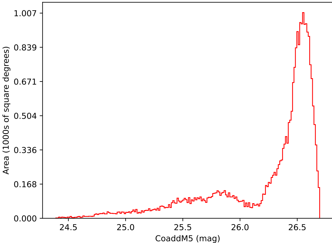
ddf_loaded_half_fl4_v3.4_10yrs All sky i band: CoaddM5
