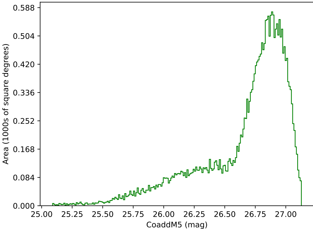
ddf_loaded_half_fl4_v3.4_10yrs All sky g band: CoaddM5
