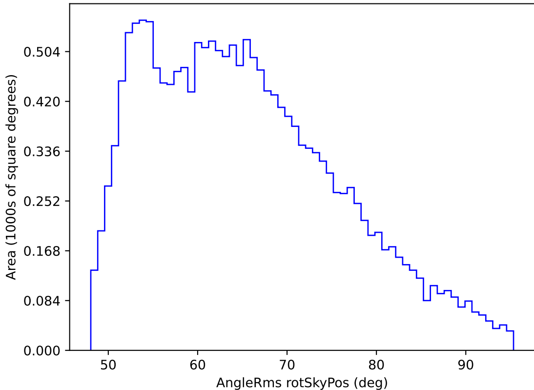
ddf_loaded_half_fl4_v3.4_10yrs WFD z band: AngleRms rotSkyPos
