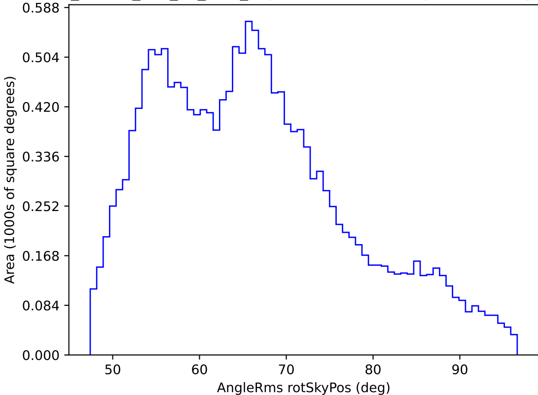
ddf_loaded_half_fl4_v3.4_10yrs WFD r band: AngleRms rotSkyPos
