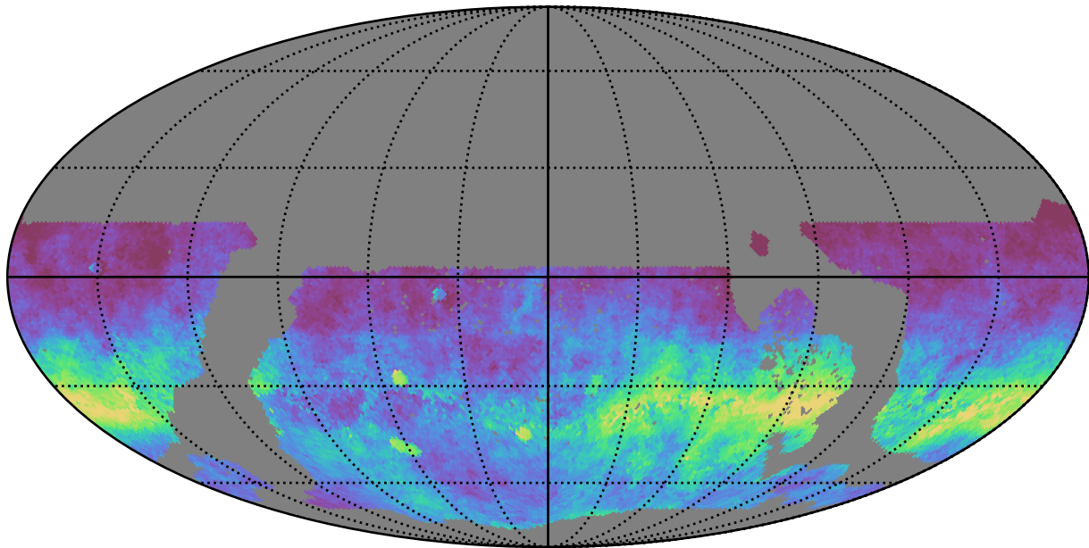
ddf_loaded_half_fl4_v3.4_10yrs WFD i band: AngleRms rotSkyPos
