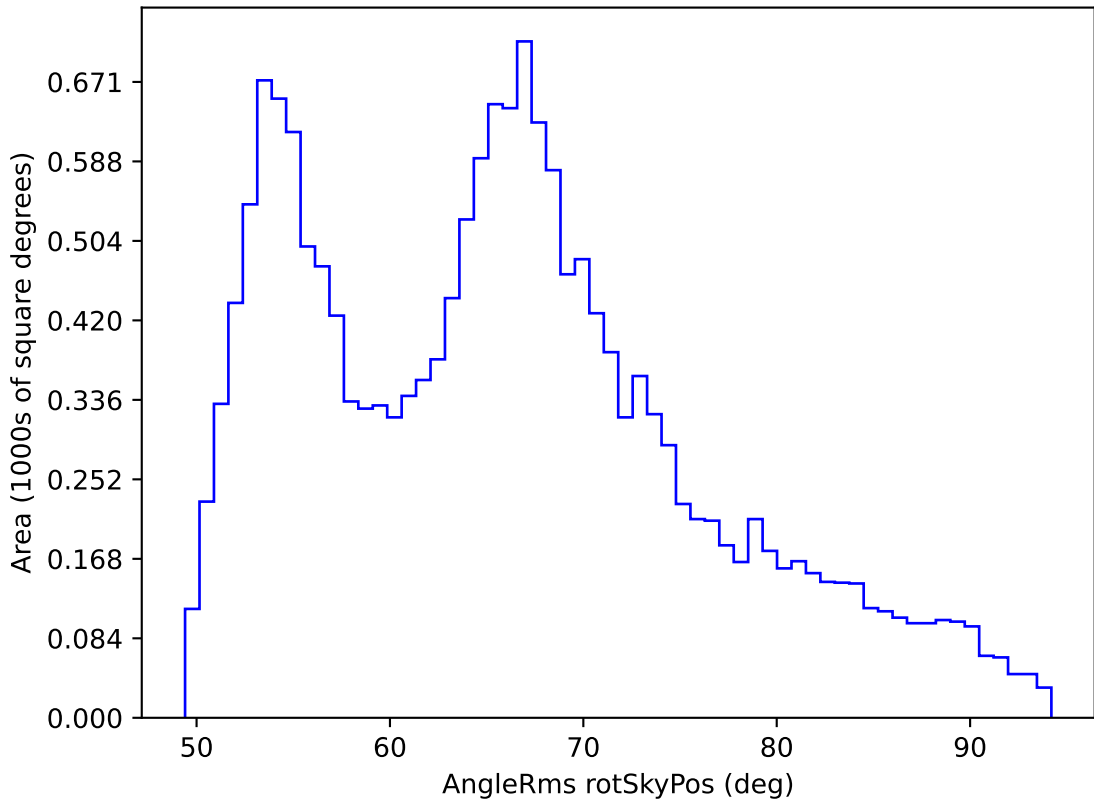
ddf_loaded_half_fl4_v3.4_10yrs WFD all bands: AngleRms rotSkyPos
