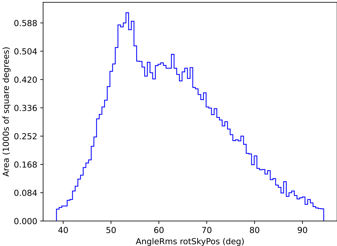
ddf_loaded_half_fl4_v3.4_10yrs All sky z band: AngleRms rotSkyPos
