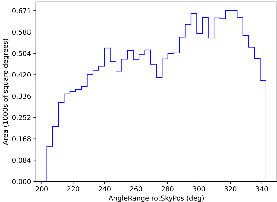
ddf_loaded_half_fl4_v3.4_10yrs WFD z band: AngleRange rotSkyPos
